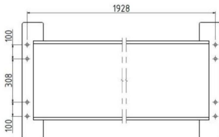
5.5.5 CRS4000 dimensions in mm
